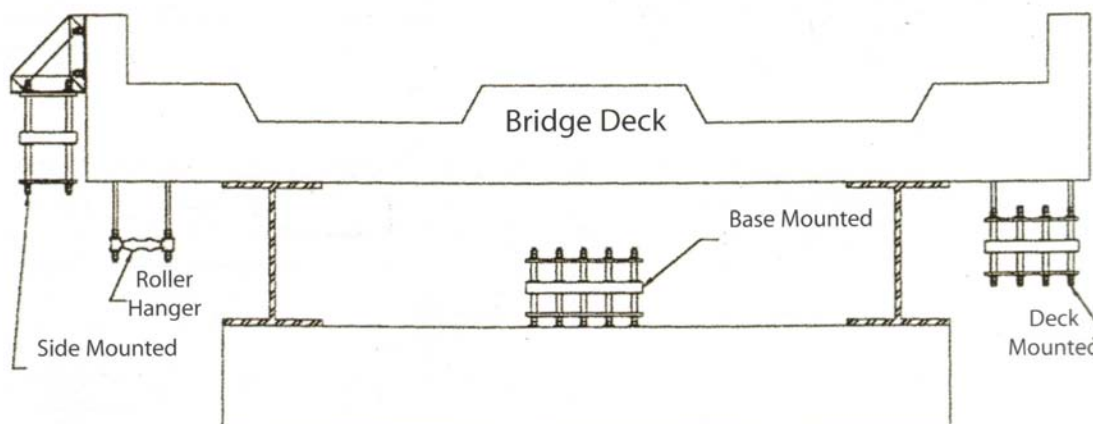
Cross Section of Typical Bridge
